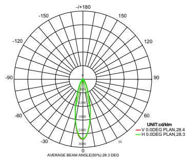
Beam angle: 30°
