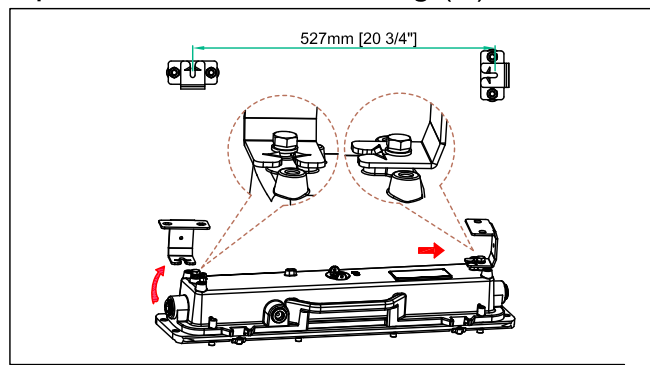
Option 8: Bracket Mounting (E):
